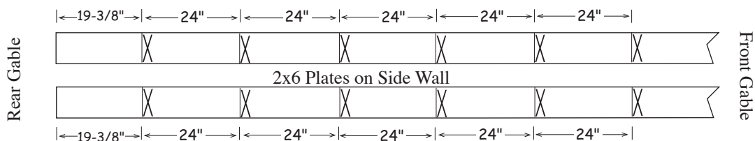
Detail 'A'
