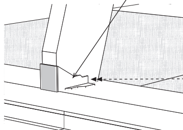
2x6 Metal Hanger
